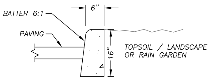
VERTICAL CURB
