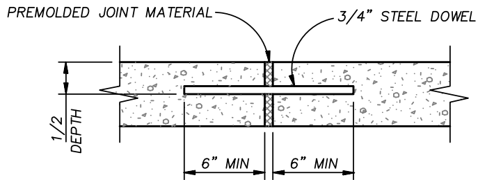
TYPICAL ISOLATION (COLD) JOINT WITH DOWEL
